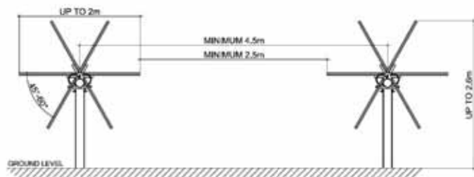
INSET B - TYPICAL TRACKER SECTION
