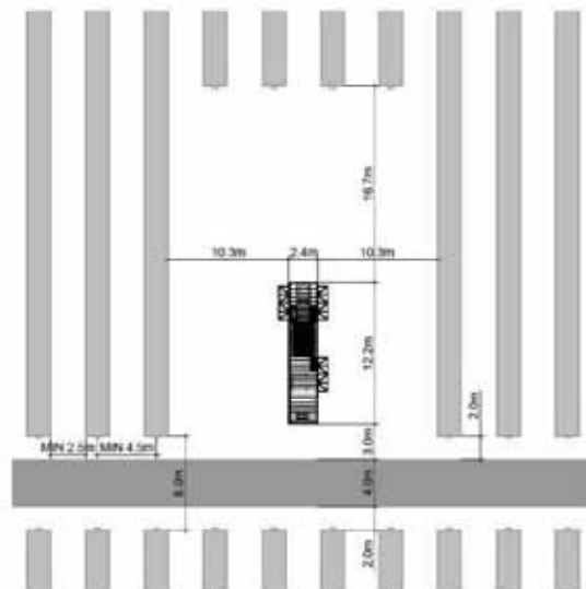
INSET A - TYPICAL INVERTER BLOCK
