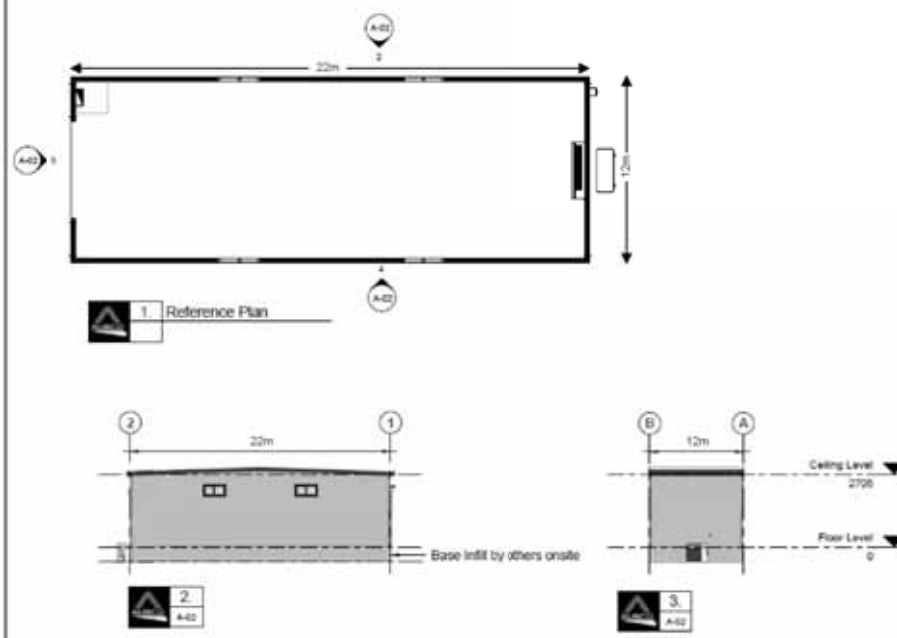
INSET F - OPERATIONS & MAINTENANCE BUILDING
